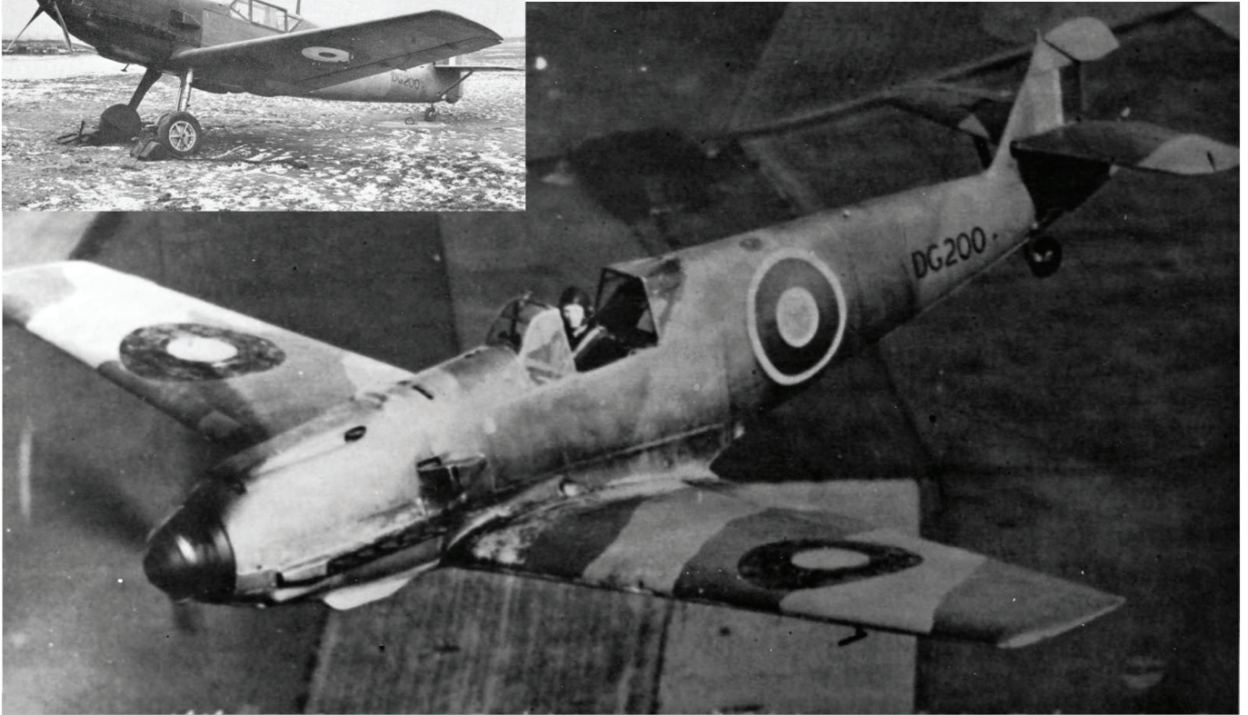
▼ Bf 109 E-4/B, W.Nr 4101, DG200 - during flying tests, Boscombe Down, February - March 1942
